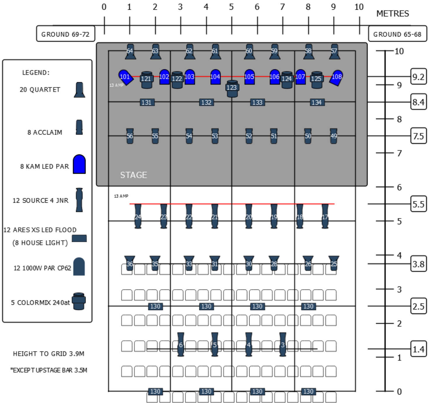
STUDIO THEATRE GENERIC RIG 2019
